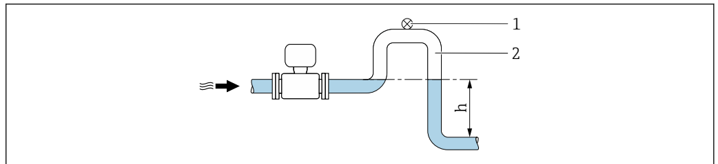
24 Installation in a down pipe
