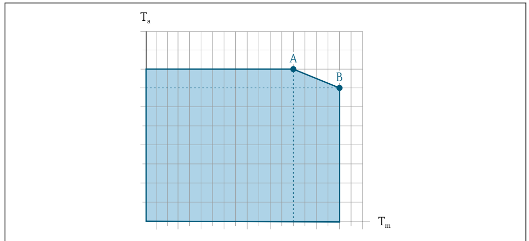
28 Exemplary representation, values in the table below.
