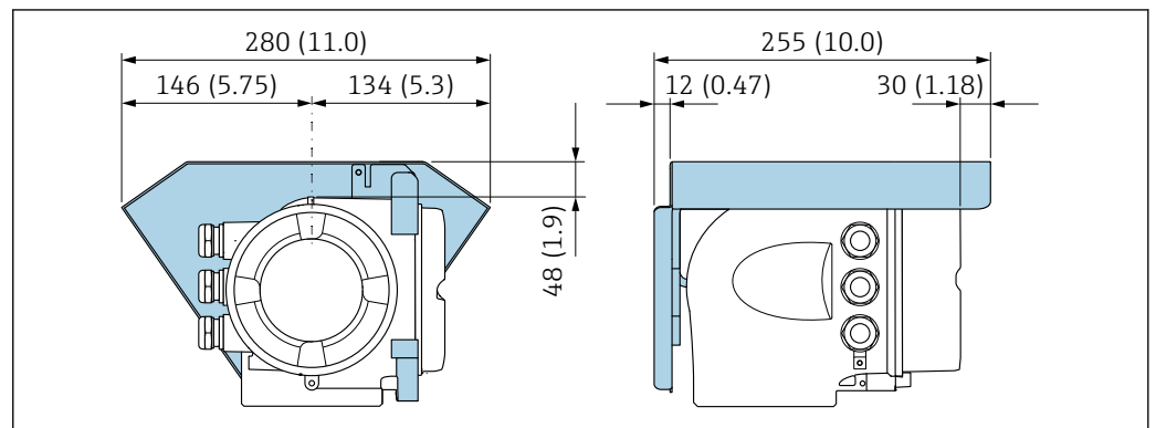
27 Weather protection cover for Proline 500
