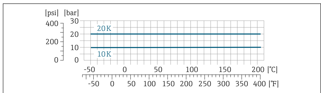
31 With flange material 1.4301 (304); wetted parts: zirconium 702, tantalum
