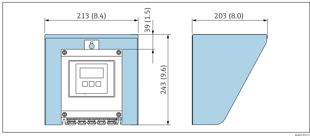
33 Weather protection cover for Proline 500 – digital
