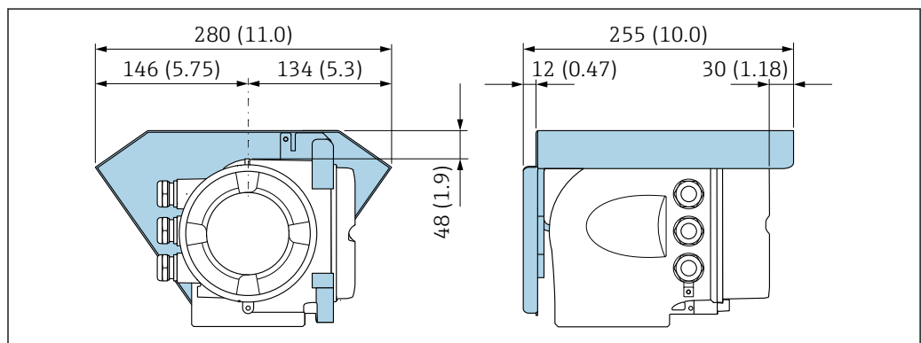
40 Weather protection cover for Proline 500
