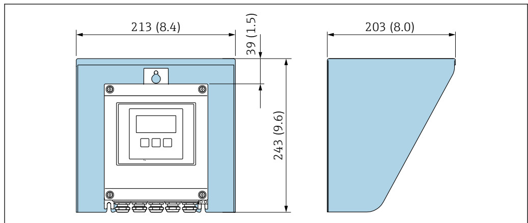
39 Weather protection cover for Proline 500 - digital
