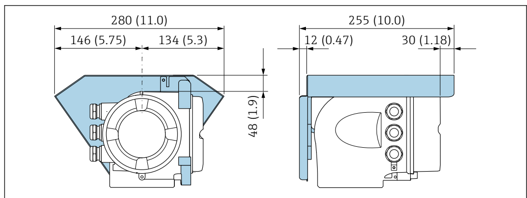
34 Weather protection cover for Proline 500
