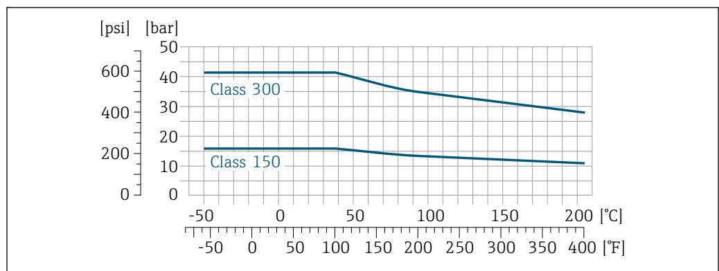
30 With flange material 1.4301 (304); wetted parts: zirconium 702, tantalum
