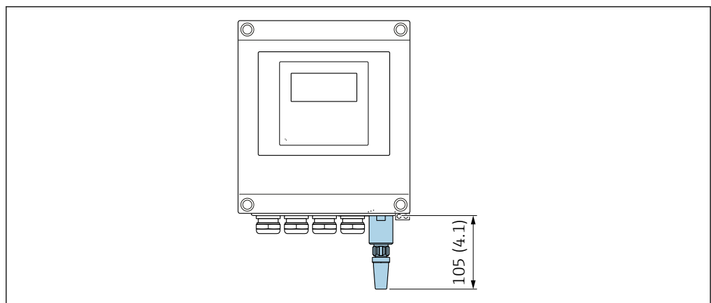
35 Engineering unit mm (in)
