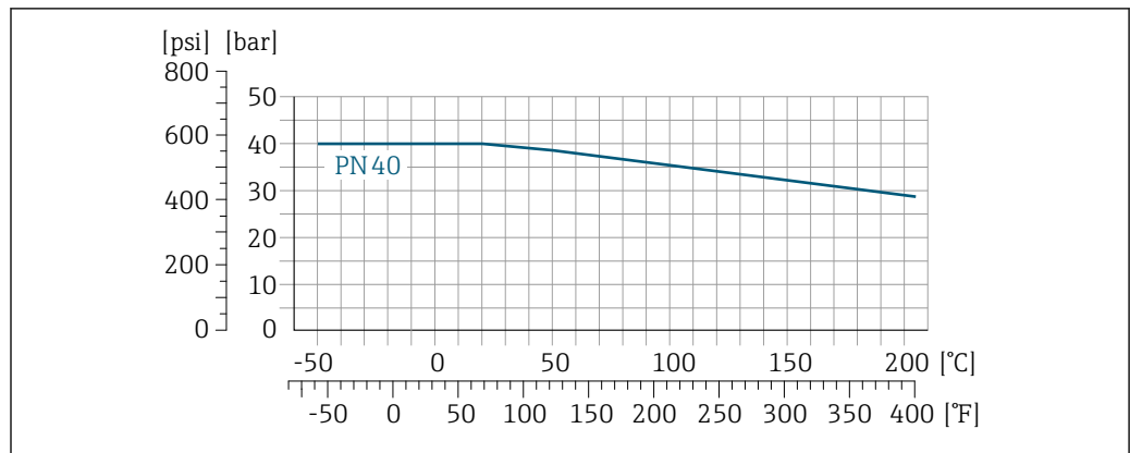
29 With flange material 1.4301 (304); wetted parts: zirconium 702, tantalum
