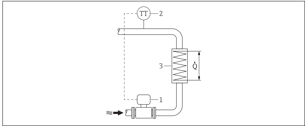
18 Layout for delta heat measurement of saturated steam and water
